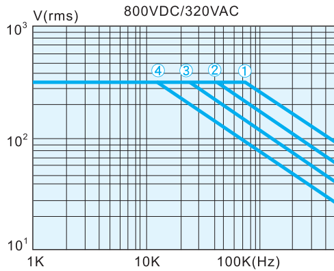
Curve:①.01 μF ②.022 μF ③.047 μF ④.1 μF
